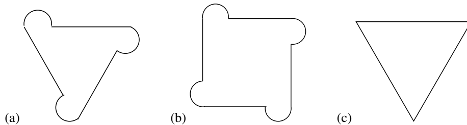
Figure 2.3: Hard wall potential with (a) symmetry Z_3 , (b) symmetry Z_4 , and (c) symmetry D_3 .
