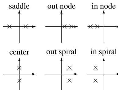
Figure 1.2: Qualitatively distinct types of exponents \{\lambda_1, \lambda_2\} of a [2 \times 2] Jacobian matrix.
