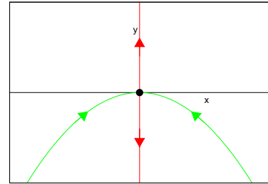
Figure 1.3: The stable/unstable manifolds of the equilibrium (x_q, y_q) = (0, 0) of 2-dimensional flow (1.49).
