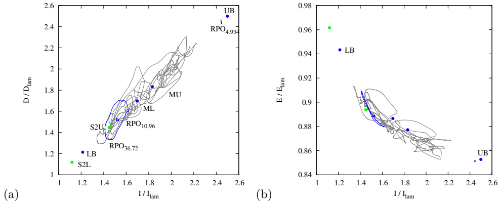
FIGURE 11. Rate of the energy input from the background pressure gradient I versus (a) the dissipation rate D , and (b) the energy E , see (2.7). Plotted are all invariant solutions of table 1, together with a typical turbulent orbit. The modulated travelling wave RPO 4.934 is visible as a little twiddle just below UB travelling wave. On the scale of these plots, the Duguet et al. (2008a) relative periodic orbit would be indistinguishable from its mother travelling wave.
