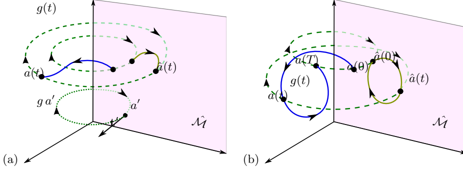
FIGURE 5. The method of slices, a state space visualisation: (a) Slice \hat{\mathcal{M}} \supset \mathcal{M}/G lies in the (d-N) -dimensional hyperplane (3.3) normal to \mathbf{t}' , where \mathbf{t}'_j span the N -dimensional space tangent to the group orbit g a' (dotted line) evaluated at the template point a' . The hyperplane intersects all full state space group orbits (green dashes). The full state space trajectory a(t) (blue) and the reduced state space trajectory \hat{a}(t) (green) are equivalent up to a ‘moving frame’ rotation a(t) = g(t) \hat{a}(t) , where g(t) is a shorthand for g(\phi(t)) . (b) In the full state space \mathcal{M} a relative periodic orbit a(0) \rightarrow a(t) \rightarrow a(T) returns to the group orbit of a(0) after time T and a rotation by g , a(0) = g a(T) . For flows with continuous symmetry a generic relative periodic orbit fills out quasi-periodically what is topologically a torus. In the slice \hat{\mathcal{M}} the symmetry-reduced orbit is periodic, \hat{a}(0) = \hat{a}(T) . This is a highly idealised sketch: A group orbit is a N -dimensional manifold, and even for \text{SO}(2) it is usually only topologically a circle (see figure 3), and can intersect a hyperplane any number of times (see figure 6 a).
