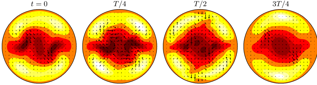
FIGURE 12. Four snapshots of relative periodic orbit \text{RPO}_{36.72} at the same fixed pipe section as in (7), reduced by the method of slices into a periodic orbit solution (see movie online ). A colormap of stream-wise velocity is shown, with white (black) indicating positive w = 0.6U (negative w = -0.7U ) velocity with respect to laminar flow. The t = 0 state has been chosen to be the closest passage (in the energy norm) to travelling wave S2U, see figure 7.
