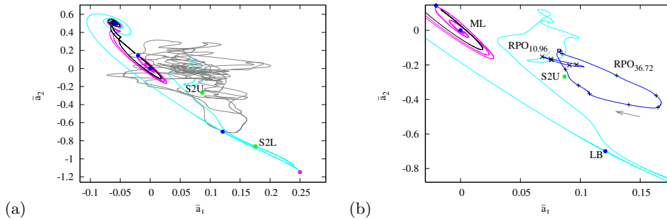
FIGURE 9. (a) Removal of the Z_2 symmetry opens the system to far more chaotic, or ‘turbulent’, transients (grey). [Compare with the same symmetry-reduced state space projection of figure 8 (b);] Within the S symmetry space, trajectories appear to frequently visit the travelling wave S2U, while the travelling wave S2L appears to be embedded in the laminar-turbulent boundary. The turbulent trajectory exhibits excursions to other states as well, most frequently ML and LB. (b) Two relative periodic orbits embedded within turbulence. Crosses are spaced every \Delta t = 2D/U on relative periodic orbit RPO_{10.96} and pluses are spaced 4D/U on relative periodic orbit RPO_{36.72} . On this scale the modulated travelling wave RPO_{4.934} [figure 8 (b), inset] only explores a region about the size of the plot dots, and plays no role in turbulent dynamics.
