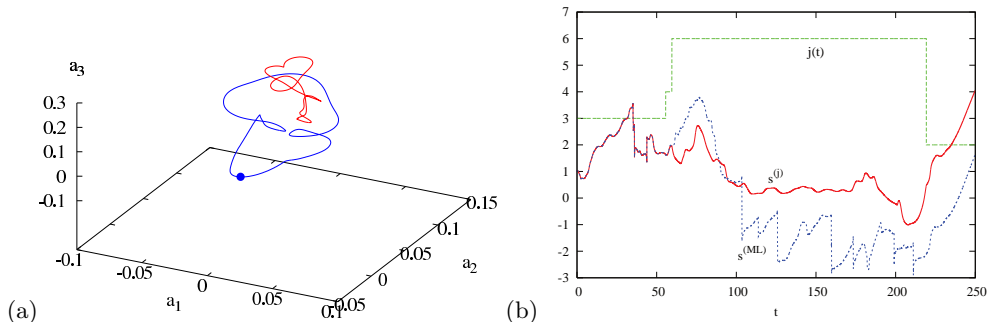
FIGURE 6. (a) Every slice hyperplane cuts every group orbit at least twice (see figure 5). An SO(2) relative periodic orbit is topologically a torus, so the two cuts are the two periodic orbit images of the same relative periodic orbit, the good close one, and the bad distant one, on the other side of slice border, and thus not in the slice. Here this is illustrated by close cut (blue) of the relative periodic orbit RPO_{36.72} torus, figure 1 (b), plotted together with the most distant cut (red), in the same slice hyperplane, but not in the slice. (b) Deviation from the mean shift, s = \ell(t) - \bar{c}t , where \bar{c} \simeq 1.274 , is estimated from a long-time simulation. The two s(t) are calculated for the same trajectory, first symmetry-reduced using a single template ML, and second, symmetry-reduced using the travelling waves in table 1 as templates indexed by j(t) ( j = 1 laminar; 2 LB; 3 ML; 4 MU; 5 UB; 6 S2U; 7 S2L). Both begin with the same template and initially experience the same jumps in the shift at t \approx 40 . By switching the template at t \approx 60 , further jumps (seen for s^{(ML)} ) are avoided in s^{(j)} .
