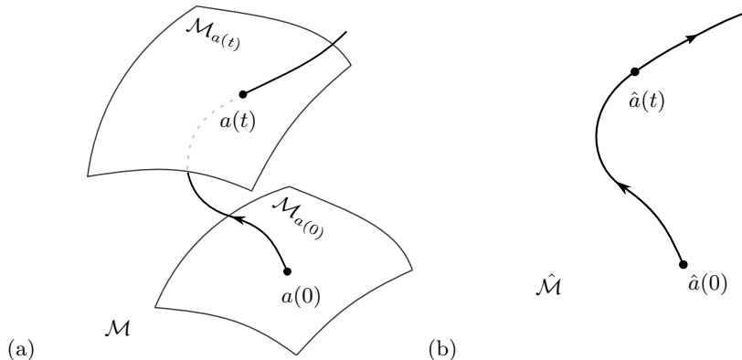
FIGURE 2. (a) The group orbit \mathcal{M}_{a(0)} of state space point a(0) , and the group orbit \mathcal{M}_{a(t)} reached by the trajectory a(t) time t later. (b) Symmetry reduction \mathcal{M} \rightarrow \hat{\mathcal{M}} replaces each full state space group orbit \mathcal{M}_a \subset \mathcal{M} by a single point in the reduced state space \hat{a} \in \hat{\mathcal{M}} .
