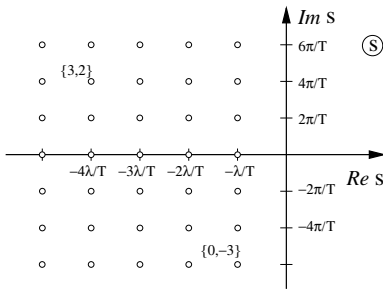
Fig. 17.3 The classical resonances \alpha = \{k, n\} (17.28) for a 2-disk game of pinball.
