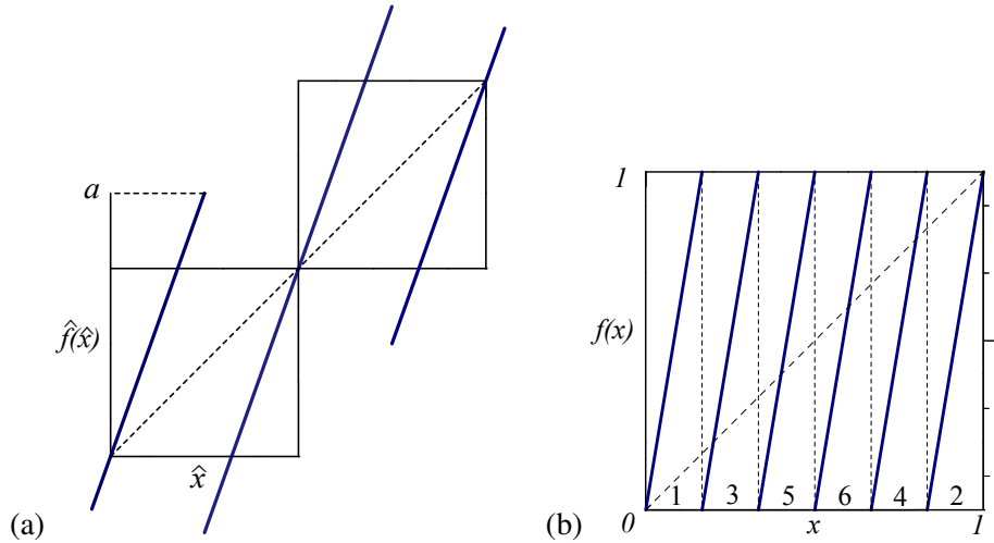
Figure 24.3: (a) \hat{f}(\hat{x}) , the full space sawtooth map (24.20), \Lambda > 2 . (b) f(x) , the sawtooth map restricted to the unit circle (24.23), \Lambda = 6 .
